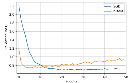
Fig. 3. The loss graphs on the validation set for different optimizers.
