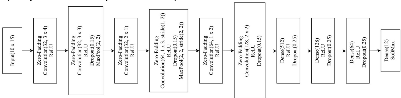
Fig. 2. CNN architecture for the classification of hand gestures.
