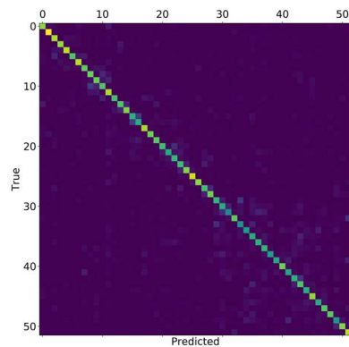
Fig. 4. Average confusion matrix constructed by the predictions of five CNNs trained with the recordings of five random subjects. Lighter colors correspond to higher values.
