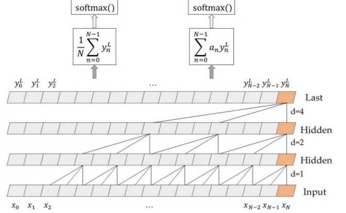
Figure 1. Graphical representation of the proposed model (Figure adjusted from [6])
