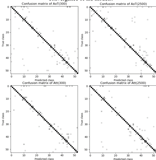
Figure 3. Average confusion matrix for each TCN model.
