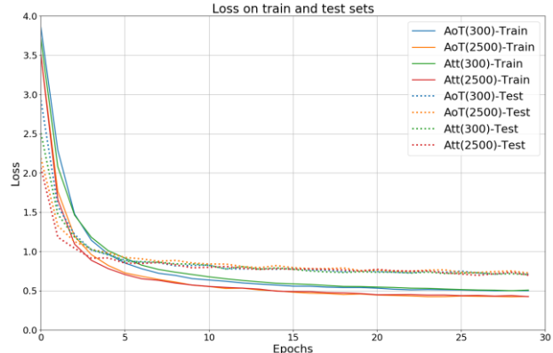
Figure 2. Average loss graphs during training and testing show convergence of the models.
